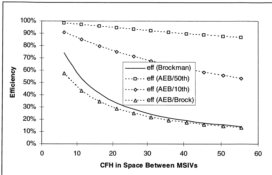
Figure 4. Brockman vs. AEB-98-03 Aerosol Removal Efficiency.
