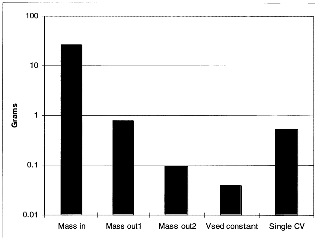
Figure 6. Mass In and Out of Steam Line.
