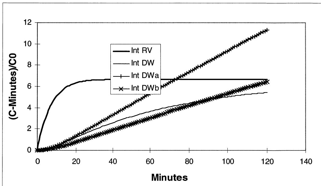
Figure 1. Integrated Concentration, Reactor Vessel vs. Drywell.
