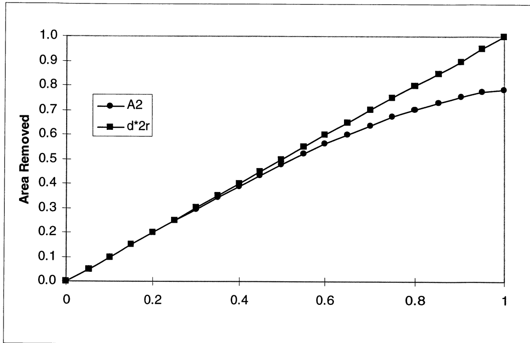
Figure 3. Comparison of A2 and \delta \cdot 2r vs. \delta for Unit Circle.
